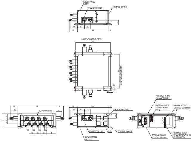
SUSPENSION BOLT: W3(W8/M10) REFRIGERANT PIPE FLARED CONNECTION
