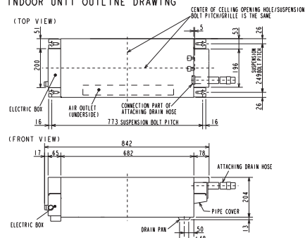
INDOOR UNIT OUTLINE DRAWING
