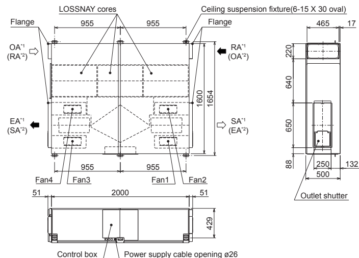
LGH-250RVXT3-E
