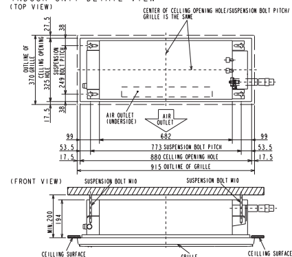
INDOOR UNIT DETAIL VIEW
