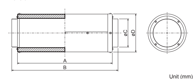
Change dimension table (Unit: mm)
