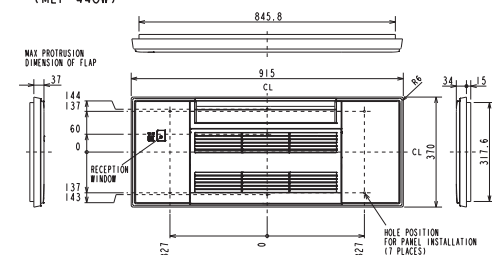
GRILLE OUTLINE DRAWING
