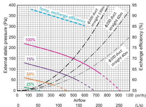
LGH-50RVS-E
